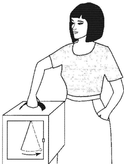
Figure 10.1: Adiabatic motion: If the case is transported very gradually, the pendulum inside keeps swinging with the same amplitude, in a plane parallel to the original one.
