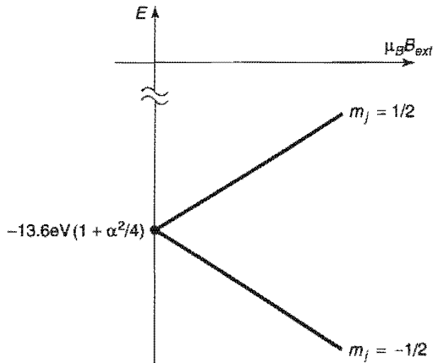
Figure 6.11: Weak-field Zeeman splitting of the ground state; the upper line ( m_j = 1/2 ) has slope 1, the lower line ( m_j = -1/2 ) has slope -1
