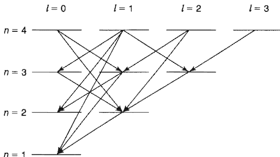
Figure 9.5: Allowed decays for the first four Bohr levels in hydrogen.
