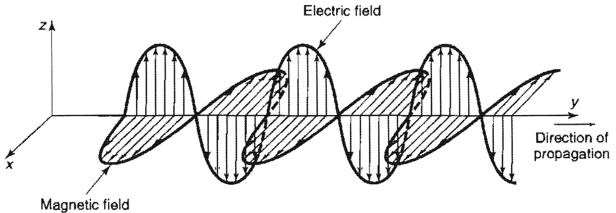
Figure 9.3: An electromagnetic wave.
