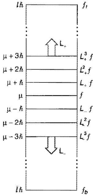
Figure 4.6: The “ladder” of angular momentum states.
